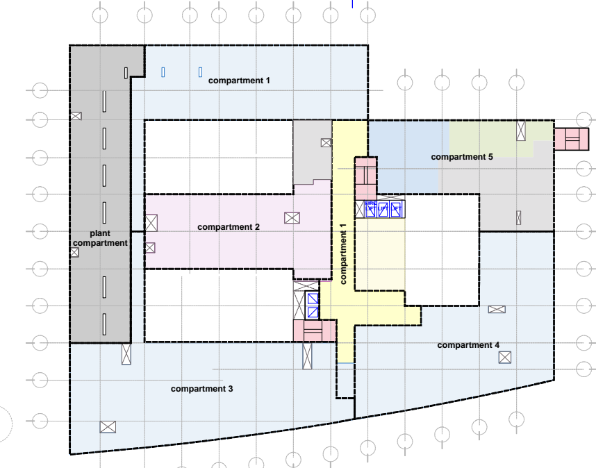
compartmentation diagram 1:500
