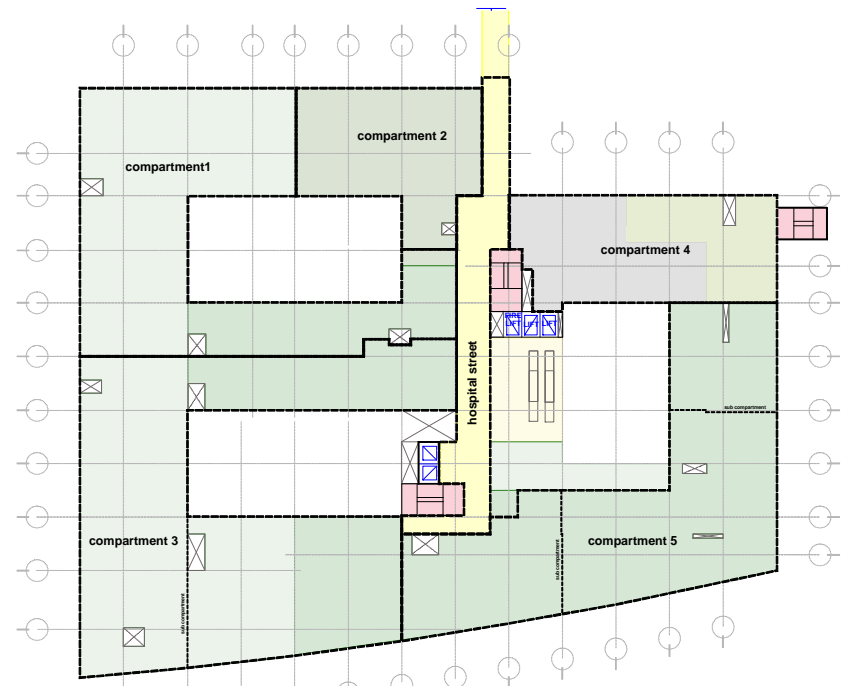
compartmentation diagram 1:500
