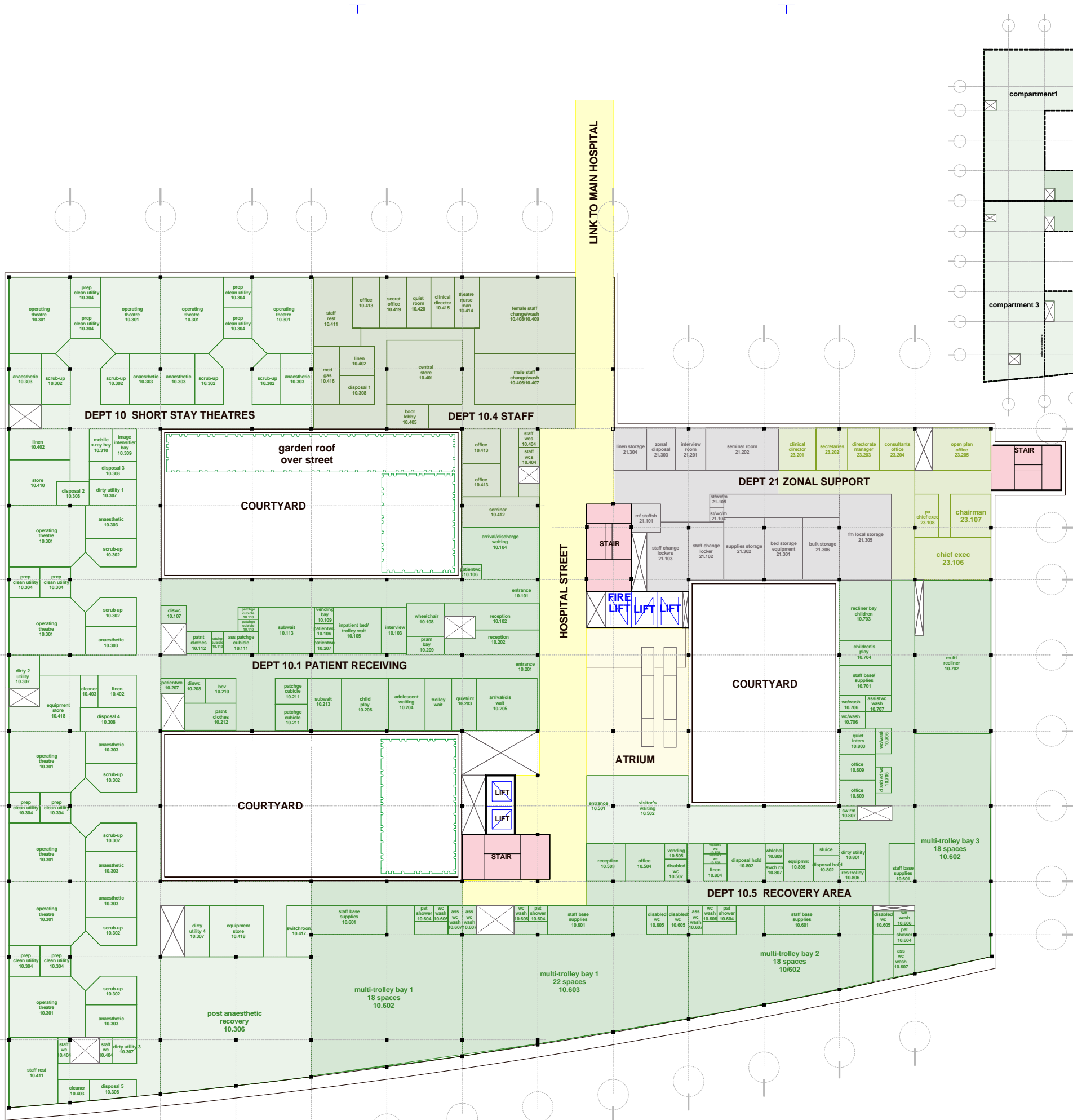
plan 1:200
