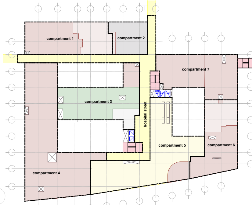
compartmentation diagram 1:500
